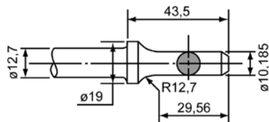
Round shank
