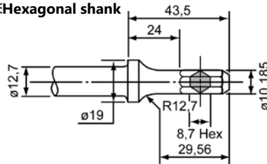
Hexagonal shank
