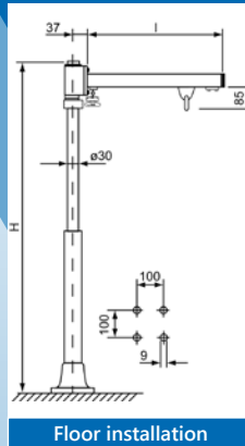
Floor installation
