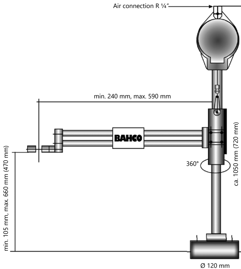
Dimensions in ( ) = Model "K"
