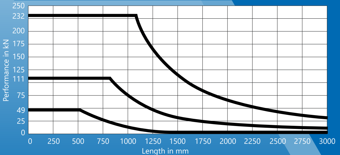
Chart of max. permitted extension / performance of CF and CF-cylinder
