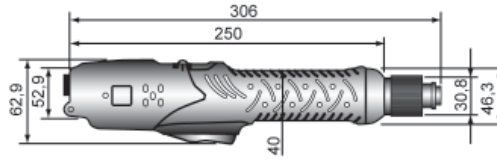
Types with lever start EA-BD630L/C EA-BD630LH/C EA-BD650L/C
