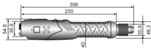
Types with pressure switch EA-BD630P/C EA-BD630PH/C EA-BD650P/C
