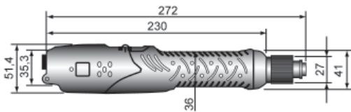
Types with pressure switch EA-BD412P/C EA-BD412PH/C EA-BD419P/C
