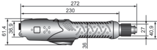
Types with lever start EA-BD412L/C EA-BD412LH/C EA-BD419L/C
